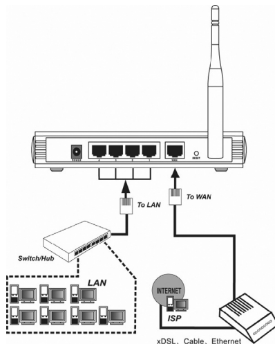
Figure 3-1 Hardware Installation of the DYWRT54 54Mbps Wireless Router
